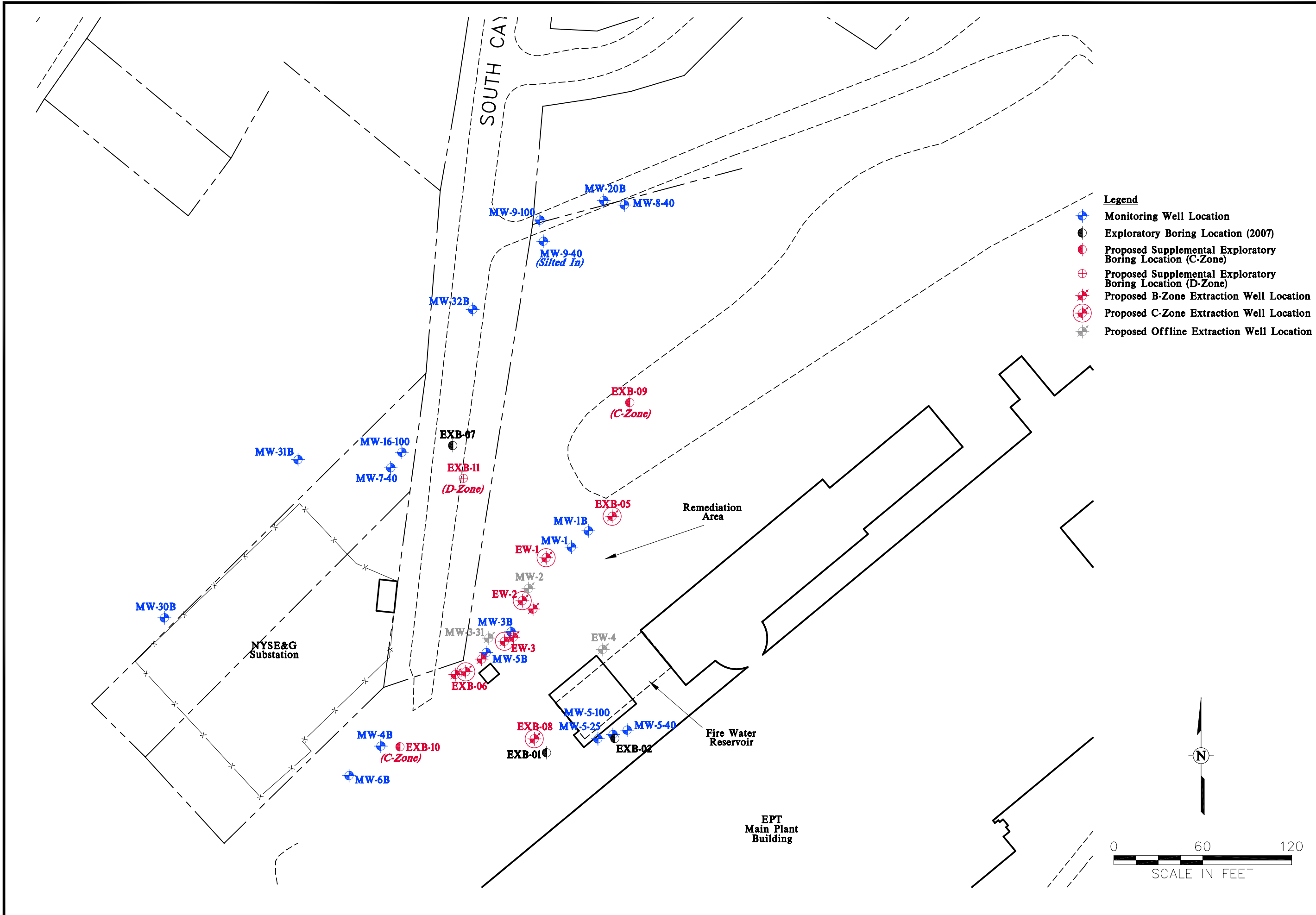
Figure 11 PROPOSED B-ZONE AND C-ZONE EXTRACTION WELL LOCATIONS
