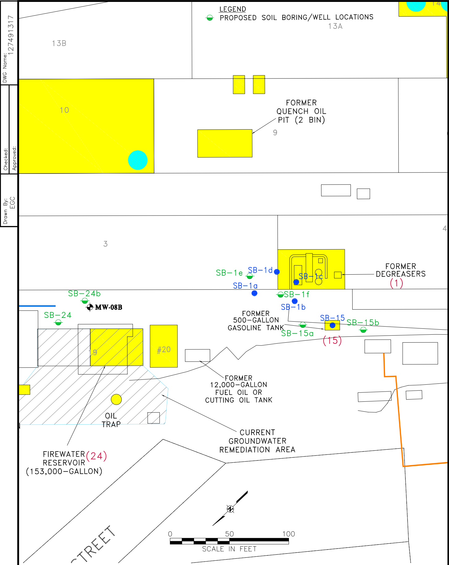
Figure 13 PROPOSED BORING LOCATIONS FOR AOC 1, 15, AND 24
