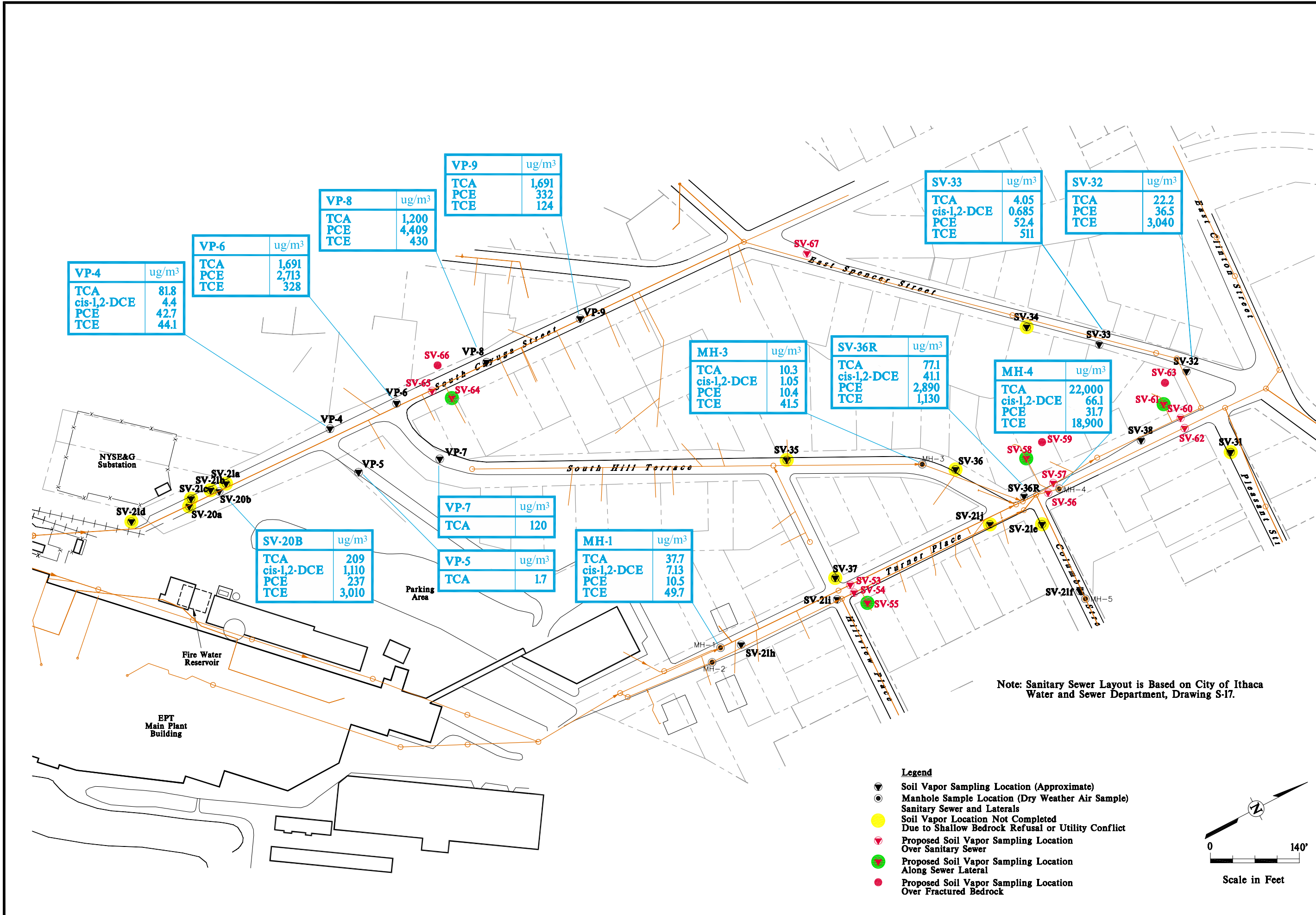
Figure 19 PROPOSED ADDITIONAL SOIL VAPOR POINT LOCATIONS
